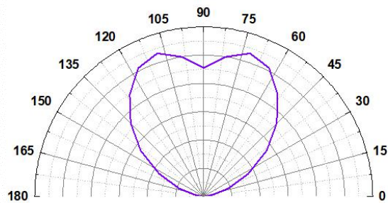
Radiation Pattern ( I_f = 40 \text{ mA} , T_a = 25 \text{ }^\circ\text{C} )
