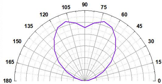
Radiation Pattern ( I_f = 80 \text{ mA} , T_a = 25 \text{ }^\circ\text{C} )
